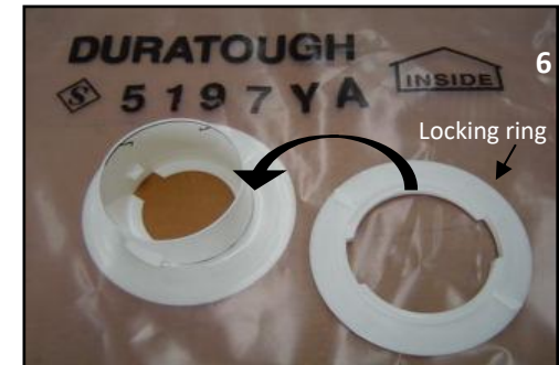
Position the locking ring over the flange base & by turning to lock it into place trapping the plastic film
