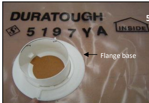
Position the first part of the Flange base as shown. The 73mm upstand should protrude into the greenhouse.
