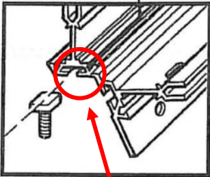
CORNER BAR
