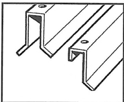
GLAZING CAPPING
