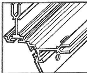
CORNER BAR
