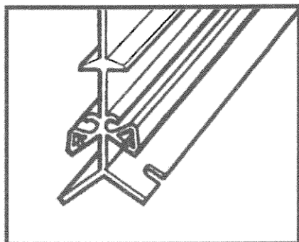
RIDGE
